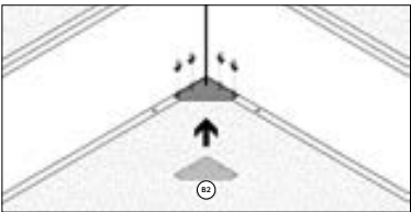
STEP 5 - Slide in foot joiner (B2), align guide holes and screw. (NB screw from below if installing on a hard surface)
